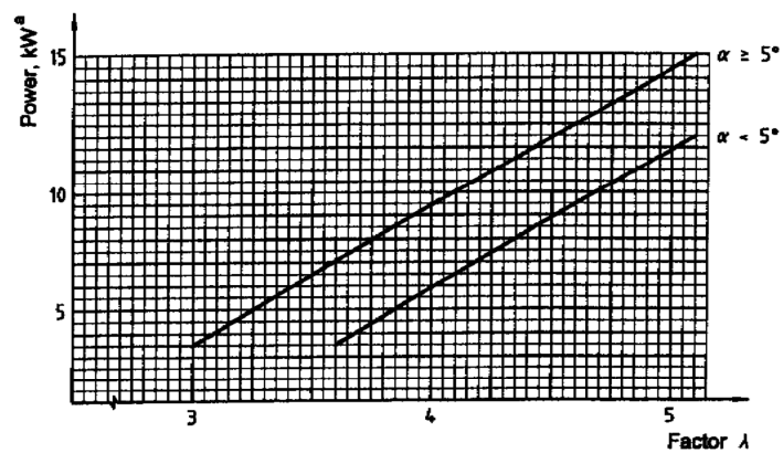
Figure C.2 — Maximum outboard capacity rating for initial testing, \lambda \leq 5,1
