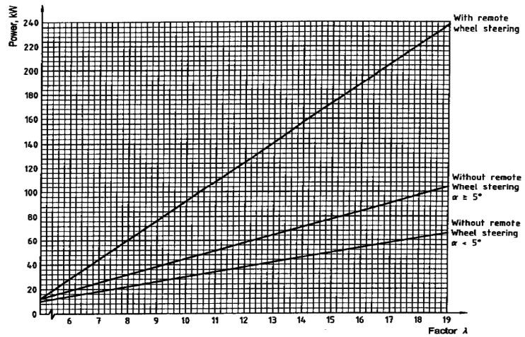
Figure C.3 — Maximum outboard capacity rating for initial testing, \lambda > 5,1
